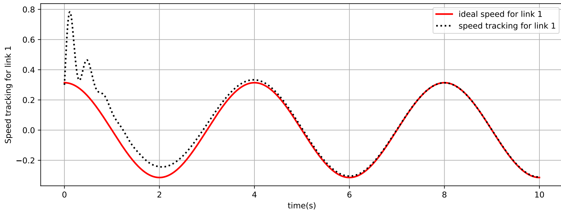
Speed Tracking Performance ( S=3 , S1=2 , m=5 )
